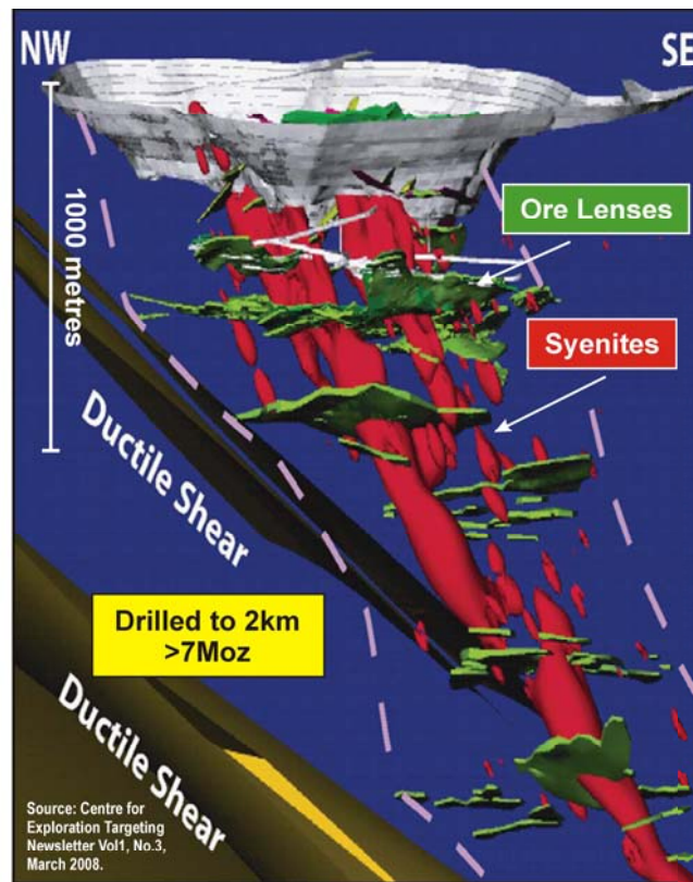
Wallaby Geological Model
